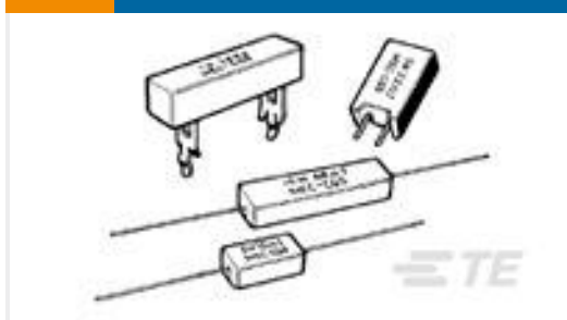
TE 产品编号1-1879009-0 SQB30 33R 5% 6.35MM FASTON
