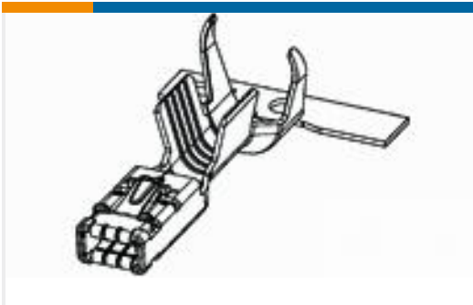
TE 产品编号1670804-3 MCON 2.8 TERMINAL - LL
