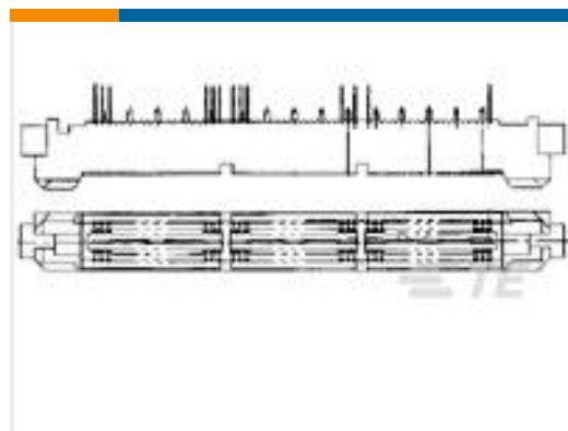
TE 产品编号767006-4 MICT,R/APLUG,152,ASY,.025,.062
