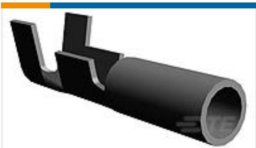
TE 产品编号1742350-1 PIN 2.08 DIA 22-18AWG TPBR
