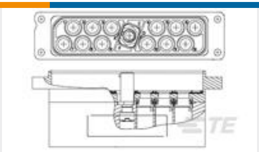
TE 产品编号1604799-5 ASY,RECEPT,PANEL MT,12 POS
