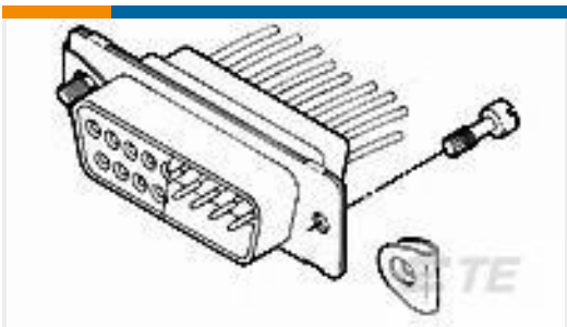
TE 产品编号1857211-1 KIT, SCREW RETAINER AMPLIMITE,
