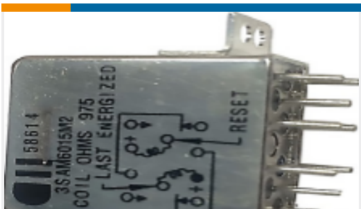
TE 产品编号3-1617522-6 3SAT1302A2=M5757/13-085
