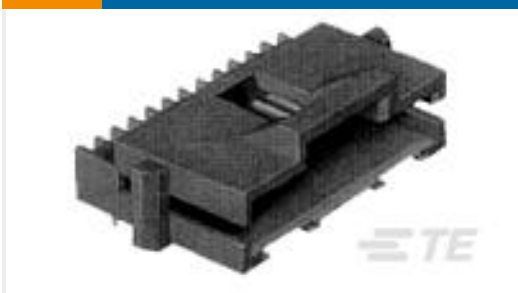
TE 产品编号1-640454-3 13P MTA100 HDR ASSY SQ STR POL
