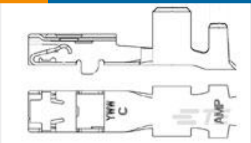
TE 产品编号1326030-7 2.8MM RECP, UNSEAL, 14-16AWG, REV
