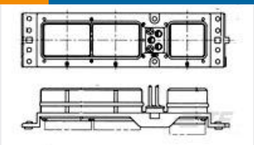
TE 产品编号1996254-1 A600,SZ2P,120T2/BLNK/85,eNi,10
