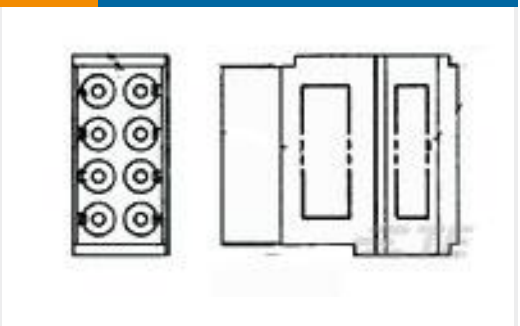
TE 产品编号592620-7 TJ, F/8/SZ 16,05 BUSSING
