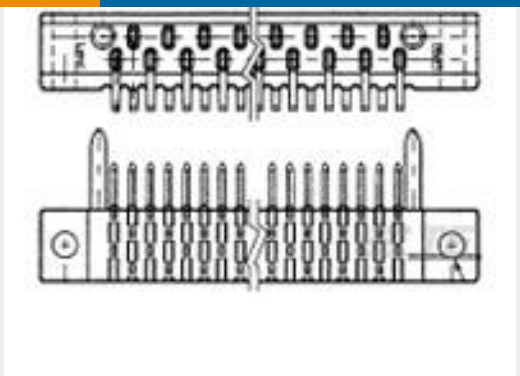
TE 产品编号2-582843-7 29 AMP BLADE HDR ASSY/MIL
