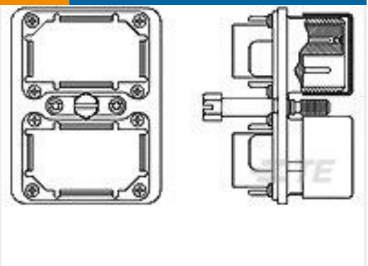
TE 产品编号207596-9 CONNECTOR, RME2P
