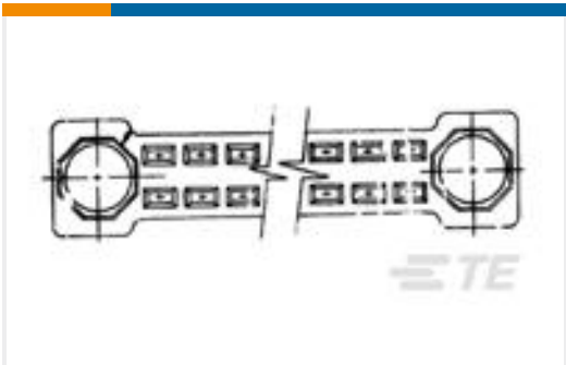
TE 产品编号1-116975-5 HSG-RECP ECONOMATE 2
