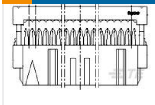
TE 产品编号1-215919-0 AMP-LATCH 15.2 HIGH TAPE
