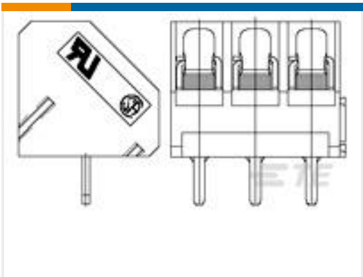
TE 产品编号1776252-2 45 degree wire inlet, 5.0mm, H
