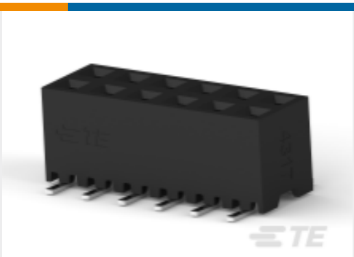
TE 产品编号1-2314844-4 14P,2MM,B-B,REC,DRVT,SMD,0.1AU, TB,W/CP
