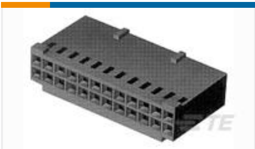
TE 产品编号280368 AMPMODU II REC. HSG, DUAL ROW, 30 POS.
