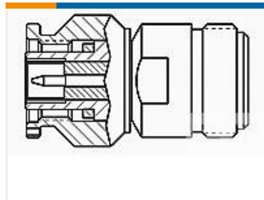
TE 产品编号 1484244-1 ADAPTER, TNC PLUG TO N JACK 3682 2311 02
