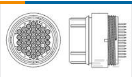
TE 产品编号788106-1 CPC POSTED PLUG ASSY, S/L, 23-37
