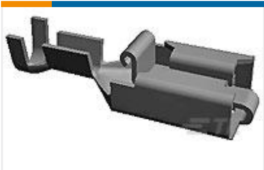
TE 产品编号154718-3 PL 250 REC 0.7-2.0 MM2 0.406 TPBR
