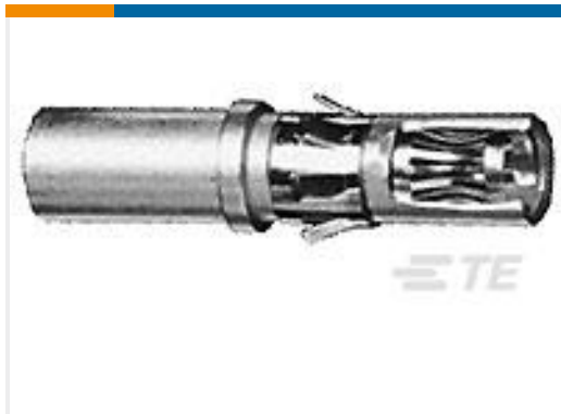
TE 产品编号193535-1 SKT ASSY. ,POWER, #12-14 AWG
