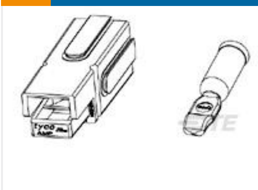
TE 产品编号1604002-5 120A SGL POLE KIT, 2 AWG RED
