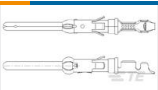
TE 产品编号1-163085-1 SPEC. PLATED
