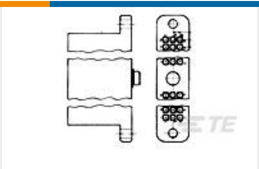
TE 产品编号204734-2 48 POS. RECPT ASSY.
