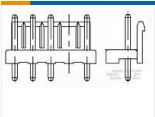
TE 产品编号1744105-2 3.96 EPHDR ASSY 5P OMIT #2 PIN
