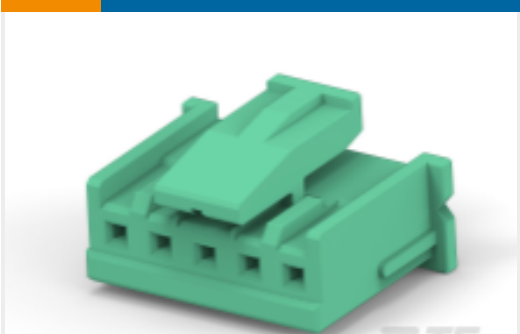
TE 产品编号8-2338183-5 EP 2.5 HOUSING 5P, GREEN, UL version
