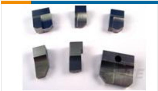
TE 产品编号1333209-1 ANVIL, COMBINATION (.130)
