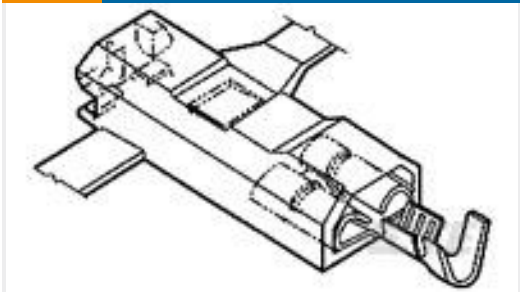
TE 产品编号1969104-1 ULTRA-POD 250 ASSY REC 18-14 AWG BR
