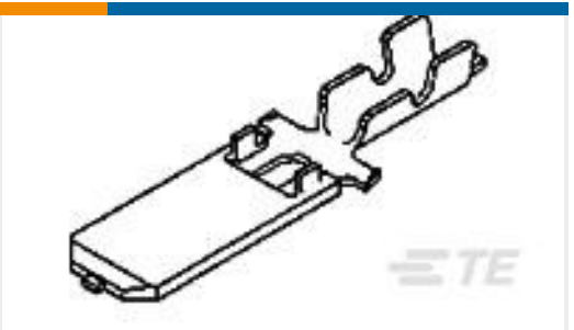
TE 产品编号170340-3 FF 250 TAB 20-14AWG PTBR WITHOUT LATCH
