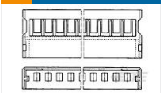
TE 产品编号917572-4 1.5 B-T-W PLUG HSG 4P BLACK
