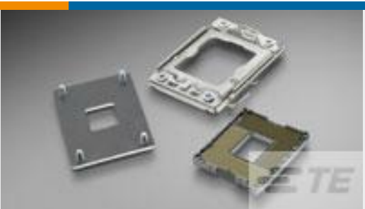
TE 产品编号2201068-1 ILM ASSY WITH COVER, LGA2011-1
