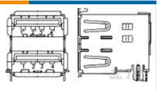
TE 产品编号1734062-3 USB Conn. stacked, offset, reel, W/ CAP
