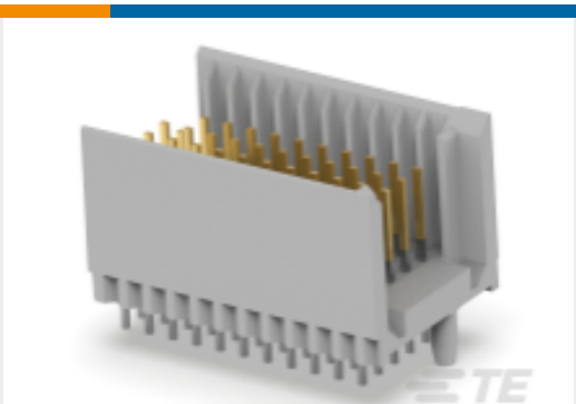
TE 产品编号2170872-1 Z-PACK TYPE/C MALE HDR 55P
