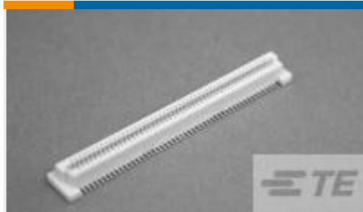
TE 产品编号2-1735482-5 0.8FH,R17H.5,120,30/Sn,TR,SC
