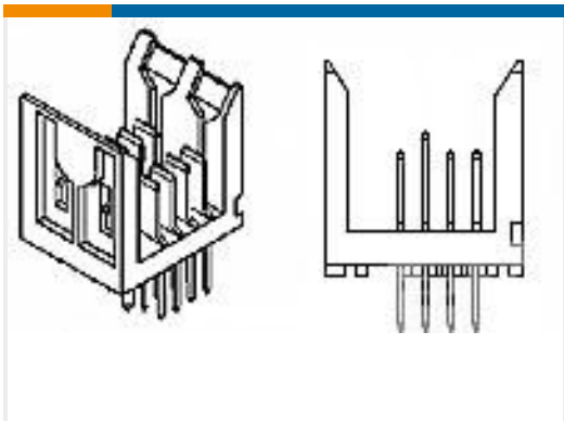
TE 产品编号5536624-1 2MM FB,ASY,008,PWR,HDR,SL,SEQ
