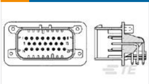
TE 产品编号1-776087-1 23 POS AMPSEAL HDR SNAP IN W/G
