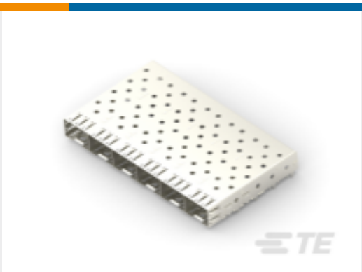
TE 产品编号1761015-3 SFP 1X6 CAGE ASSY W/ KAPTON TAPE, PF
