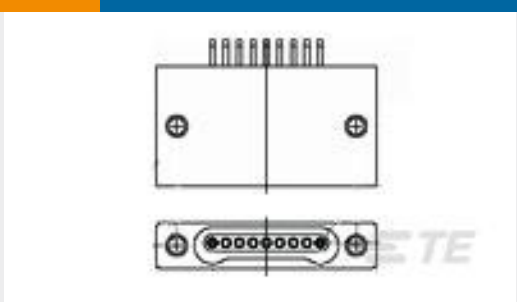
TE 产品编号1589462-9 SSL009L2HN = SMT CONN
