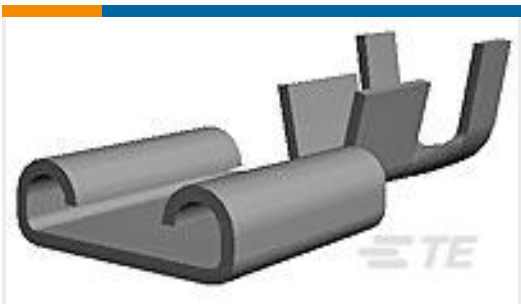
TE 产品编号1-160305-6 250 FASTON,REC.,10-12 AWG,TPBR
