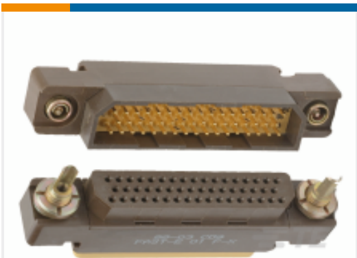
TE 产品编号ZPF000000000017891 FAST-E 03 M-X-B 00 B
