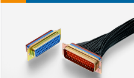
TE 产品编号2157480-4 AMPLIMITE IP67,SZ4, 109, 37 POS,IFS, PLUG
