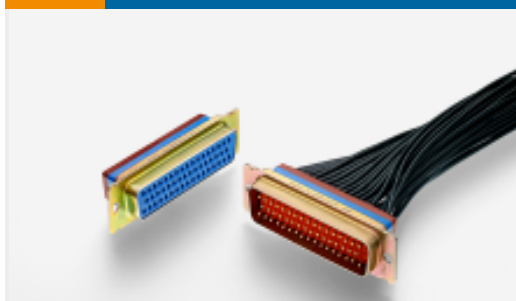
TE 产品编号1-2221760-5 AMPLIMITE IP67, SZ5, 90, 78 POS, RCPT
