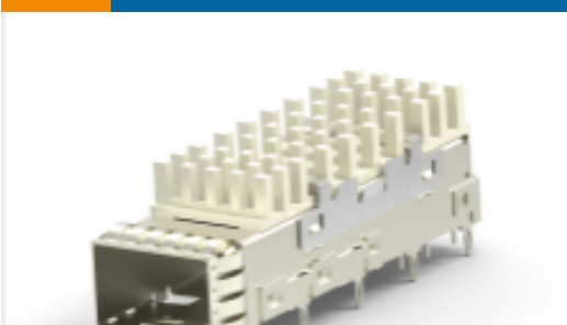
TE 产品编号2291634-2 SFP+ 1X1 CAGE ASSY, PF,WITH HEATSINK
