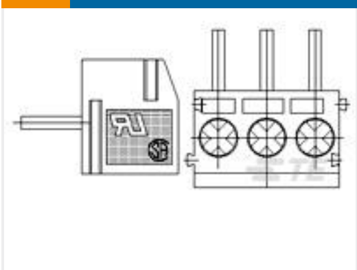
TE 产品编号1776253-8 R/A Top Wire Entry, 3.5mm, HT,
