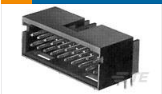
TE 产品编号102617-4 12 MODII HDR DRRA SHRD .100CL
