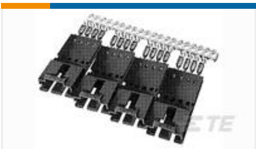
TE 产品编号2-322873-5 DG 22-16 HT ALUMEL R 6
