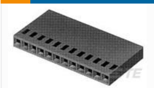
TE 产品编号3-87499-4 18 MODIV HSG COMP SR .100CL
