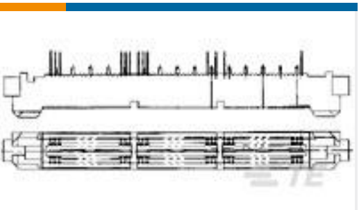
TE 产品编号 767039-3 MICTOR,RA PLUG,114,.093PCB,ASY
