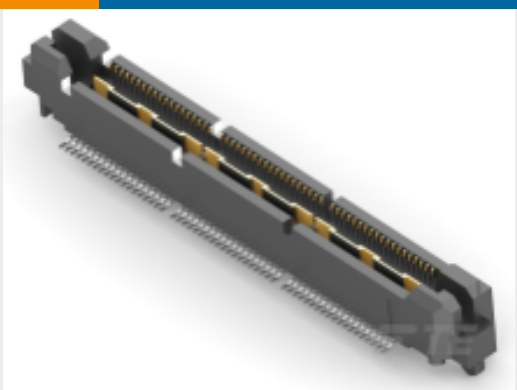
TE 产品编号 1-767007-0 MICT,260PLUG,114,ASSY,.025,REC
