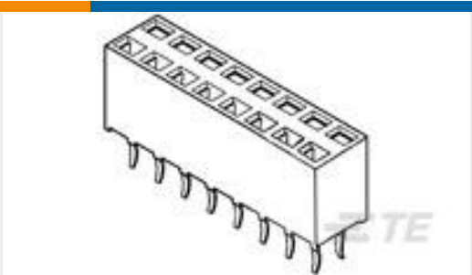
TE 产品编号215310-2 2X2P HV100 REC CON. TE, 8.5MM,TIN
