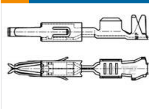
TE 产品编号1241730-2 MT3 REC 1.6 Contact SWS Sn
