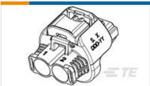
TE 产品编号1544978-3 RECEPT HSG ASSY, 8MM NG1+, 2W, SEALED
