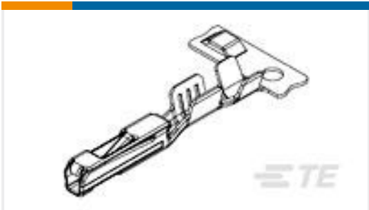
TE 产品编号1326028-2 0.64MM FEMALE CONTACT,AU, 22AWG
