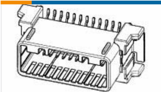
TE 产品编号1717396-1 0.64 SMD 16P CAP ASSEMBLY V-TYPE.
