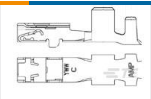
TE 产品编号1326030-6 2.8MM RECP,UNSEAL,18-20,REVREE
