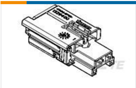
TE 产品编号1326490-3 4P JPT/MT3 PLUG W/LATCH,GRAY
